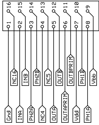
P1 16-pin DIP Plug
